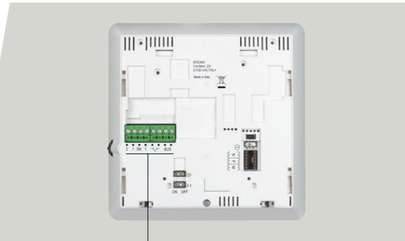
BTicino 2 wires video indoor units have standard plug-in SCS BUS clamps: maximum simplicity.
